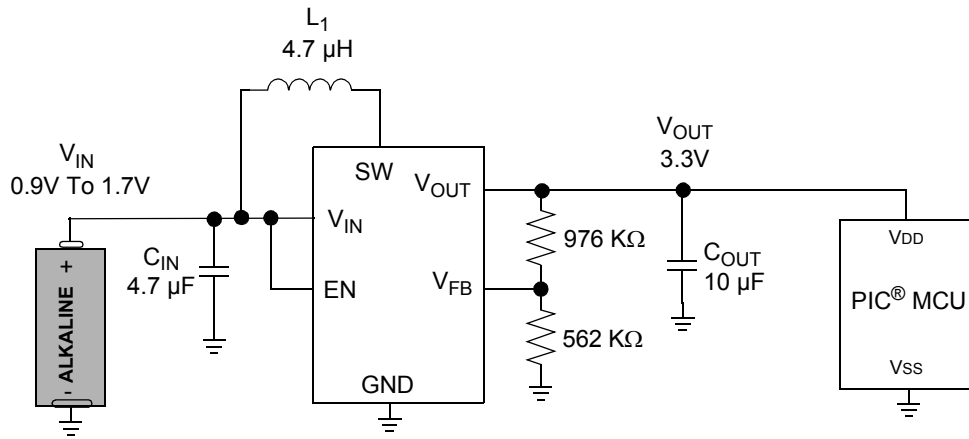
MCP1623/24 Typical Application Circuit
