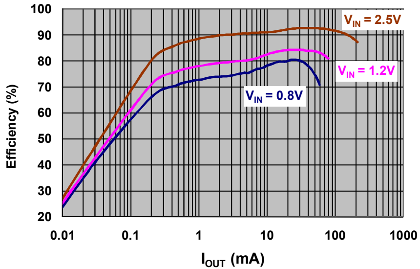
MCP1624 Efficiency vs. I_{OUT} , V_{OUT} = 3.3V
