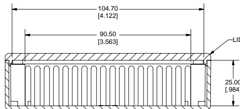
SECTION C-C SCALE 1 : 1
