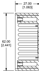
SECTION B-B SCALE 1 : 1
