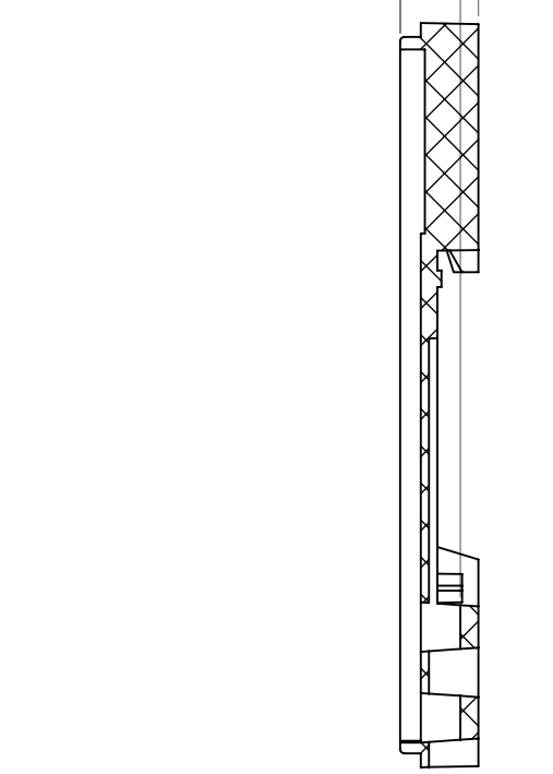
SECTION B-B SCALE 1 : 1
