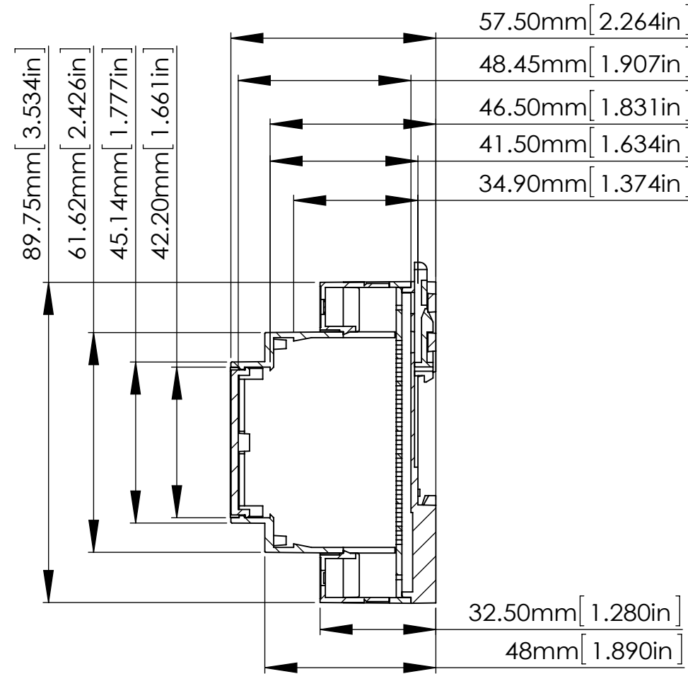
SECTION B-B SCALE 2:3
