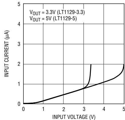
Figure 4. Input Current
