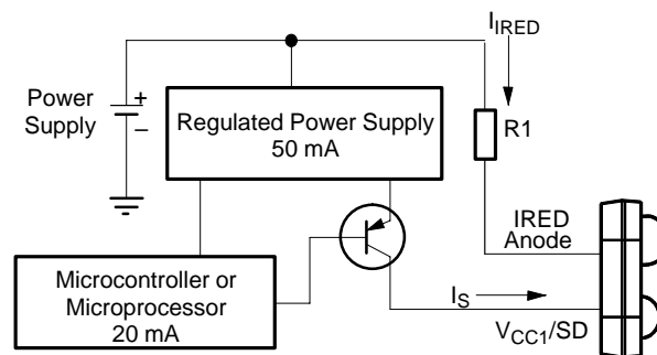
TFDU4100 (Note: Typical Values Listed) Receive Mode
