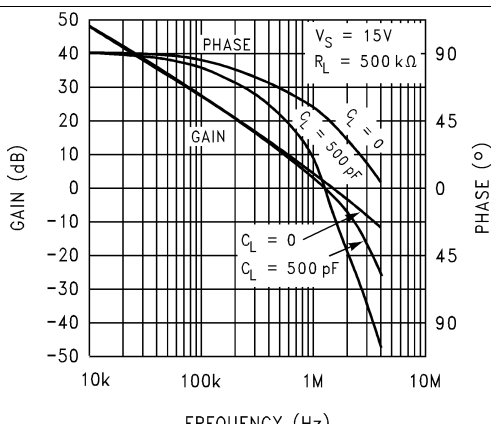
Figure 30. Gain and Phase vs Capacitive Load
