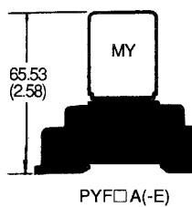
Mounting height of relay with socket
