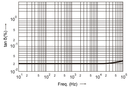
Dissipation Factor V.S. Frequency (Typical Values)
