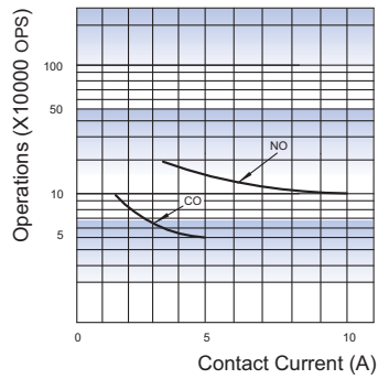
ENDURANCE CURVE
