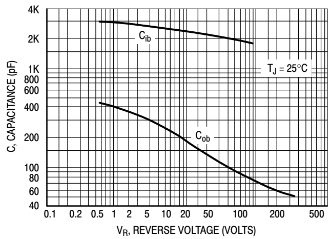
Figure 10. Capacitance
