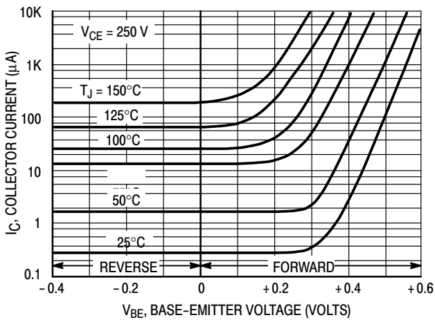
Figure 9. Collector Cutoff Region
