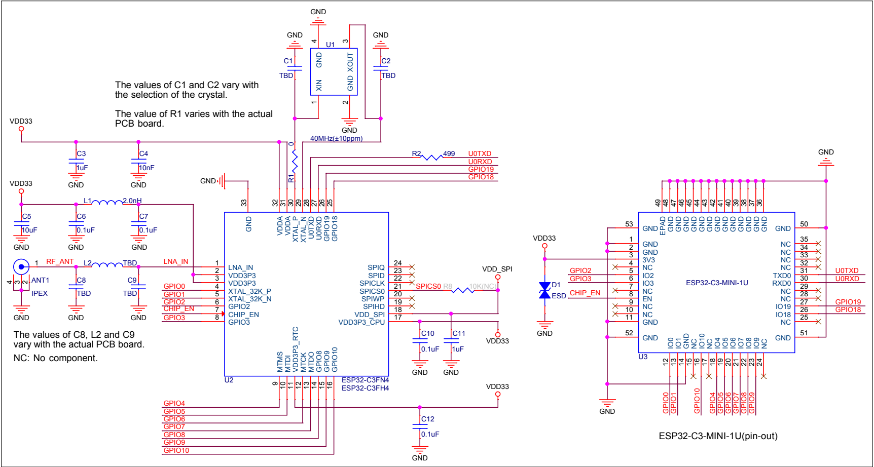
Figure 6: ESP32-C3-MINI-1U Schematics
