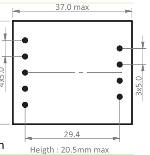
EVD 30 reinforced insulation creepage distances: 6mm
