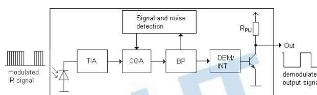
Block Diagram
