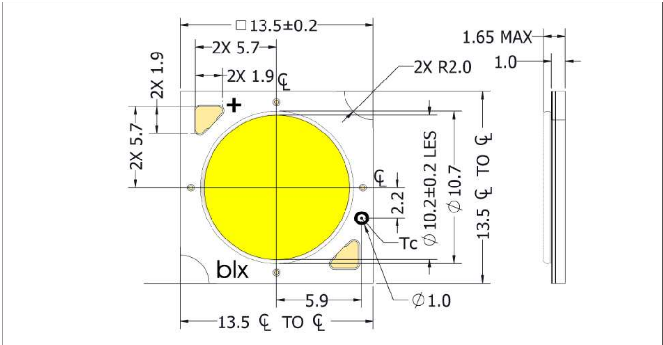
Figure 11: Drawing for V10 LED Array
