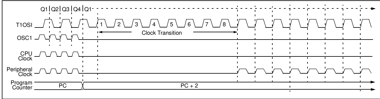
FIGURE 3-5: TIMING TRANSITION FOR ENTRY TO SEC_IDLE MODE
