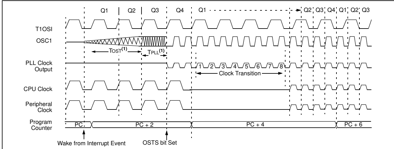
FIGURE 3-6: TIMING TRANSITION FOR WAKE FROM SEC_RUN MODE (HSPLL)
