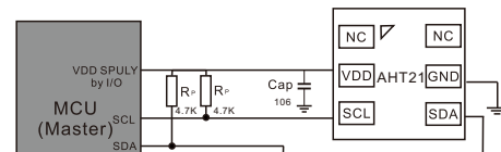
Figure 15 Typical application circuit, the pull-up voltage and VDD of SCL and SDA are powered by the MCU.
