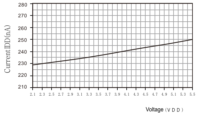
Figure 7 shows the typical relationship between supply current and voltage (dormancy mode) at 25 °C. Please be noted that the deviation between these data and the display value may reach ± 50 % of the display value. At 60 °C, the coefficient is about 15. (Compared with Table 2).
