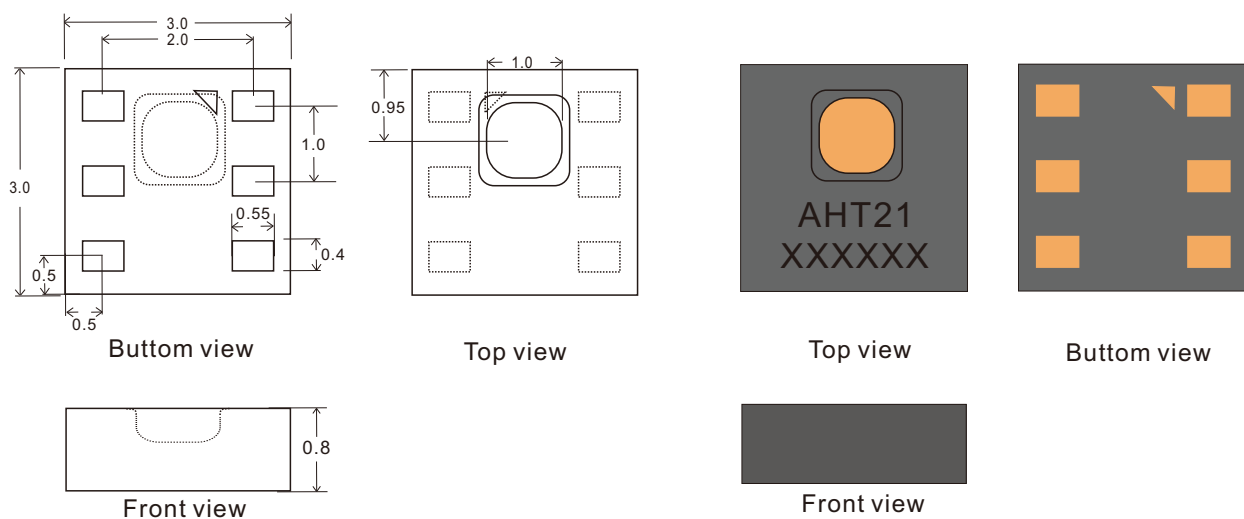
Figure 1: AHT21 Sensor Package Diagram (Unit: mm Tolerance: ±0.1 mm)
