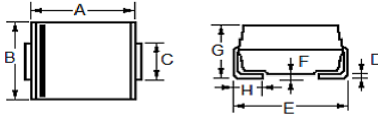
DO-214AB (SMC) Surface mount plastic package
