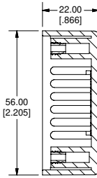
SECTION B-B
