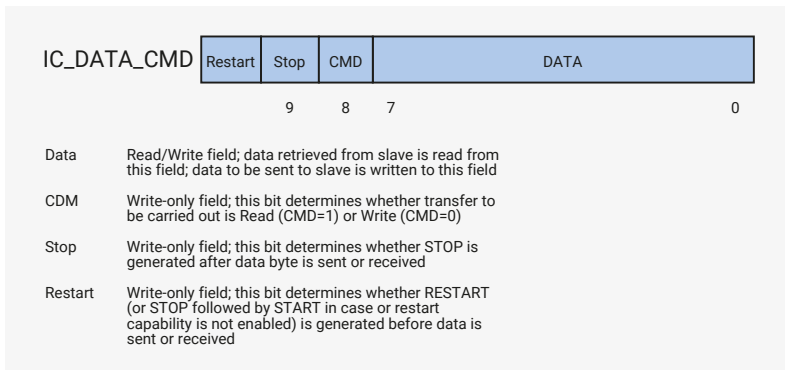
Figure 75. IC_DATA_CMD Register
