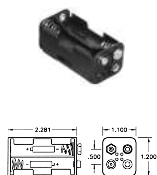
Holds Four (4) "AA" Cells in Series
