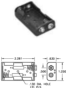
Holds Two (2) "AA" Cells in Series
