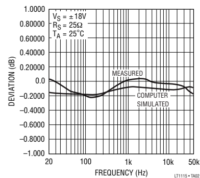
Measured Deviation from RIAA Response. Input at 1kHz = 1\text{mV}_{\text{RMS}} Pre-Emphasized
