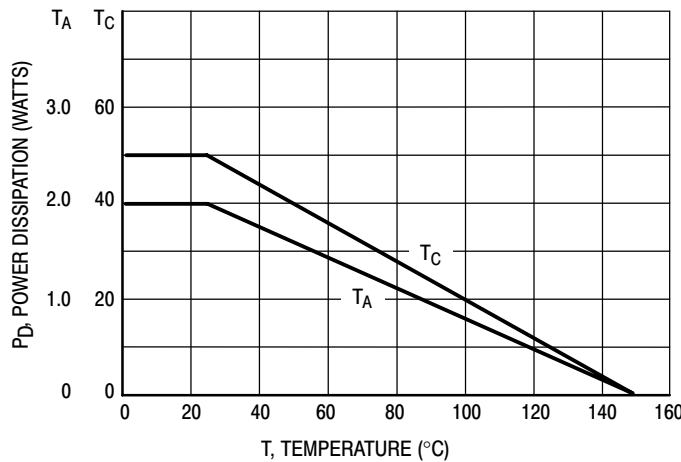
Figure 3. Power Derating
