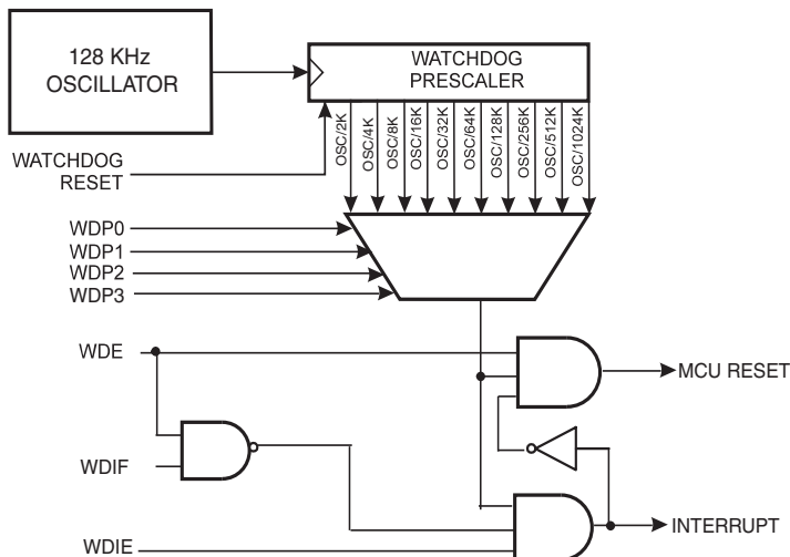
Figure 9-7. Watchdog Timer
