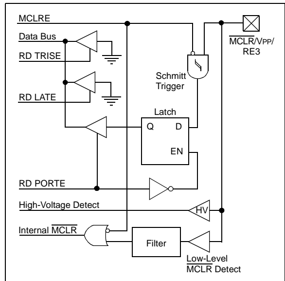
FIGURE 10-14: BLOCK DIAGRAM OF \overline{\text{MCLR}}/\text{VPP}/\text{RE3} PIN
