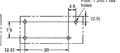
Mounting Holes (Bottom View)
