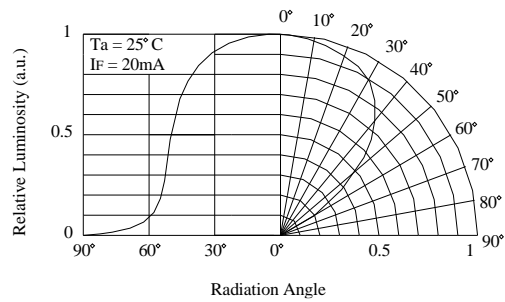
Directivity (Angle : 100^\circ )
