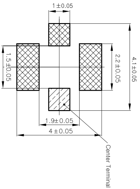
Recommended PCB Pattern
