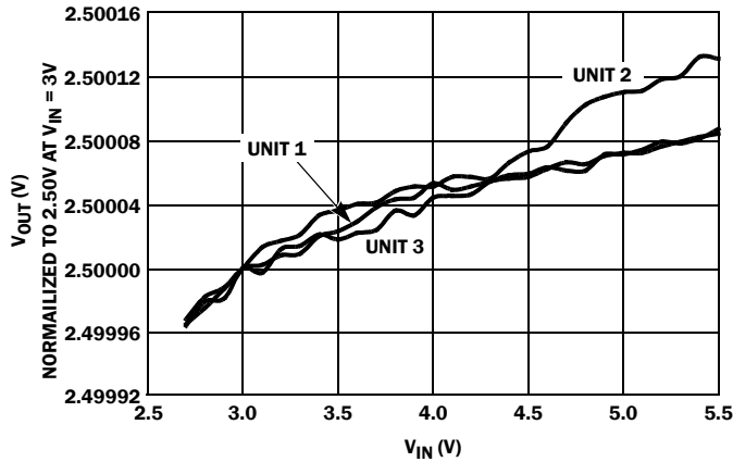
FIGURE 72. LINE REGULATION, 3 UNITS
