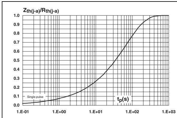
Figure 11. Relative variation of thermal impedance junction to ambient versus pulse duration (DO-21AD)
