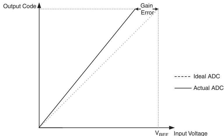
Figure 26-12. Gain Error
