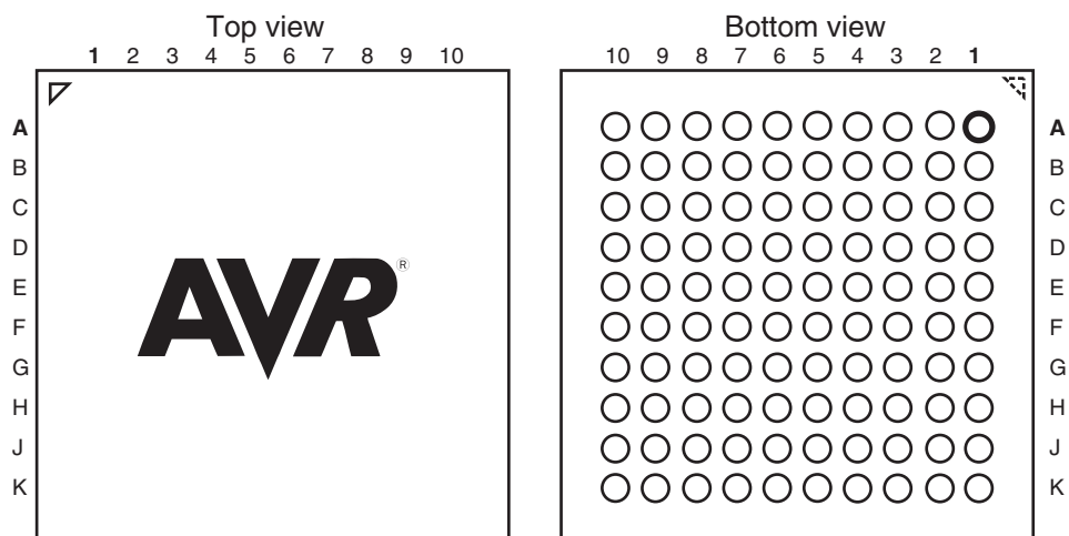
Figure 1-2. CBGA-pinout ATmega640/1280/2560
