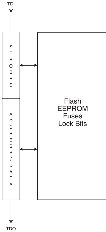
Figure 30-14. Programming Command Register
