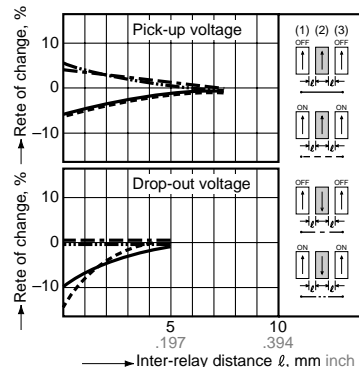
6-(1). Influence of adjacent mounting (1 Form C)
