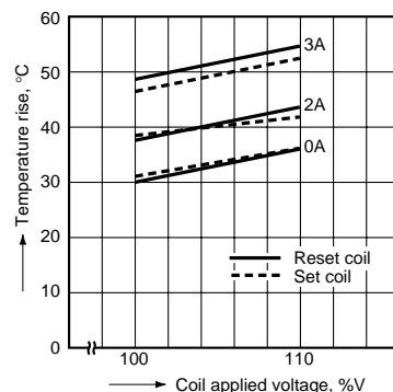
4-(3). Coil temperature rise (2 Form C 2 coil latching type) Point measured: Inside the coil Ambient temperature: 20° to 21°C 68° to 70°F
